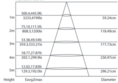
Wide Zoom Flux out: 949.5 lm
